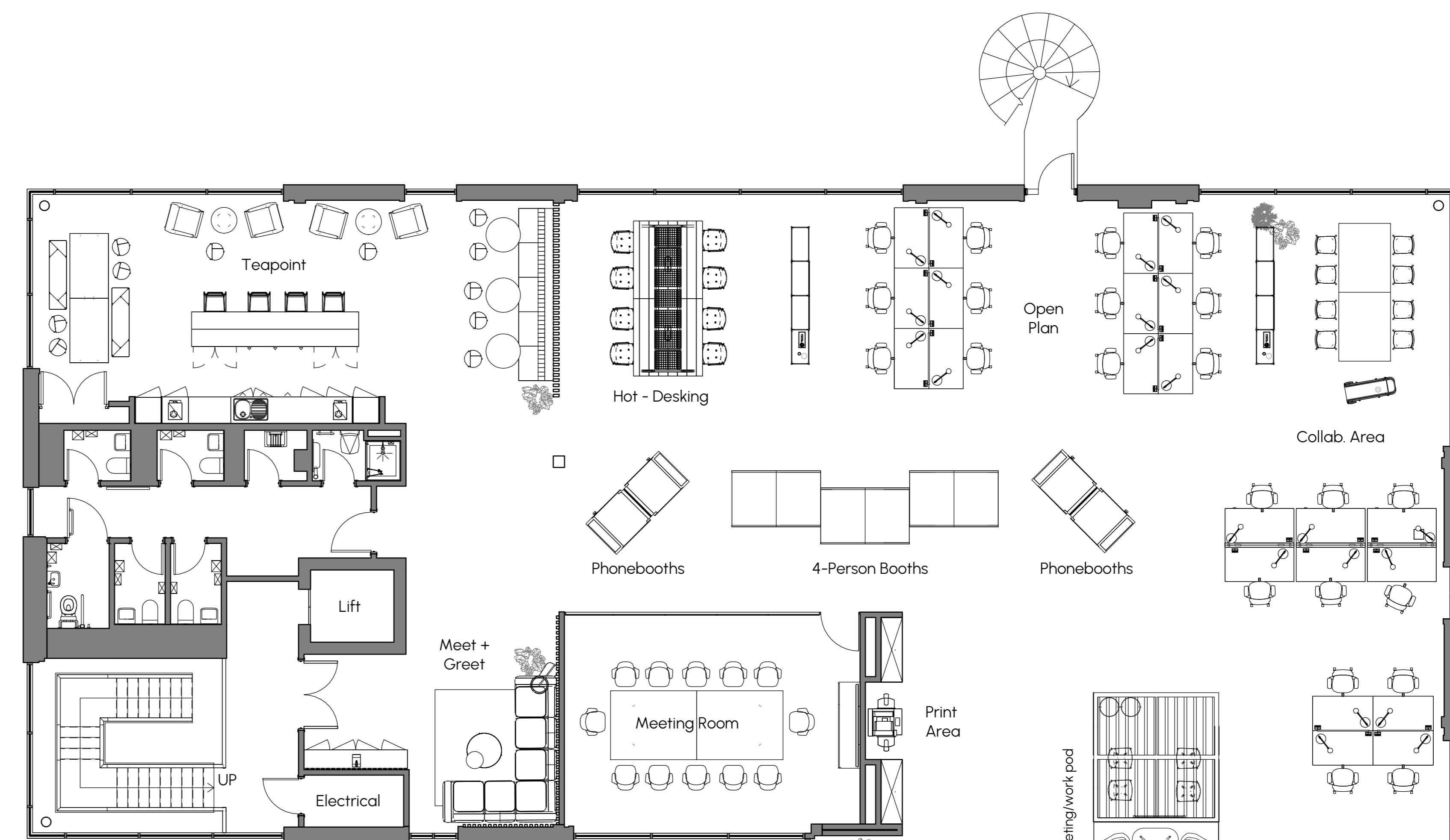
3 First Floor Proposed Layout 1:75
